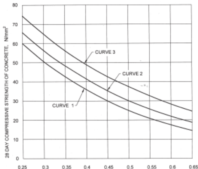
FIGURE 1: RELATIONSHIP BETWEEN FREE WATER CEMENT RATIO AND 28 DAYS COMPRESSIVE STRENGTH OF CONCRETE
